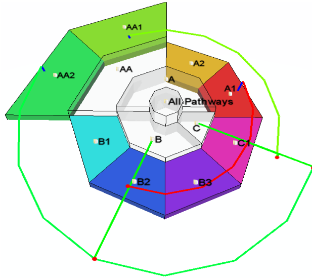
Fig 5.3 Highlight orbits of graph G2.
